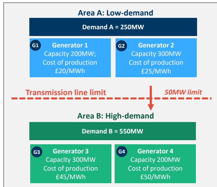
Figure 2-1: Simple two node worked example
