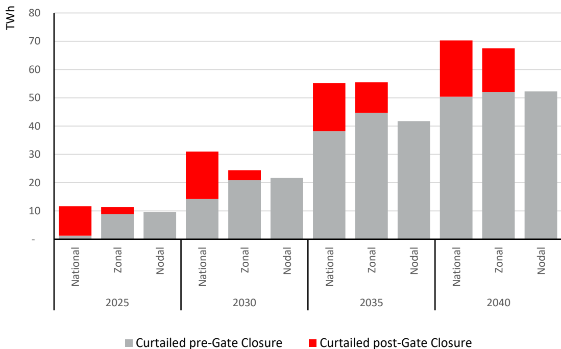
Figure 6-25: Wind curtailment – SysTr (NOA7)
