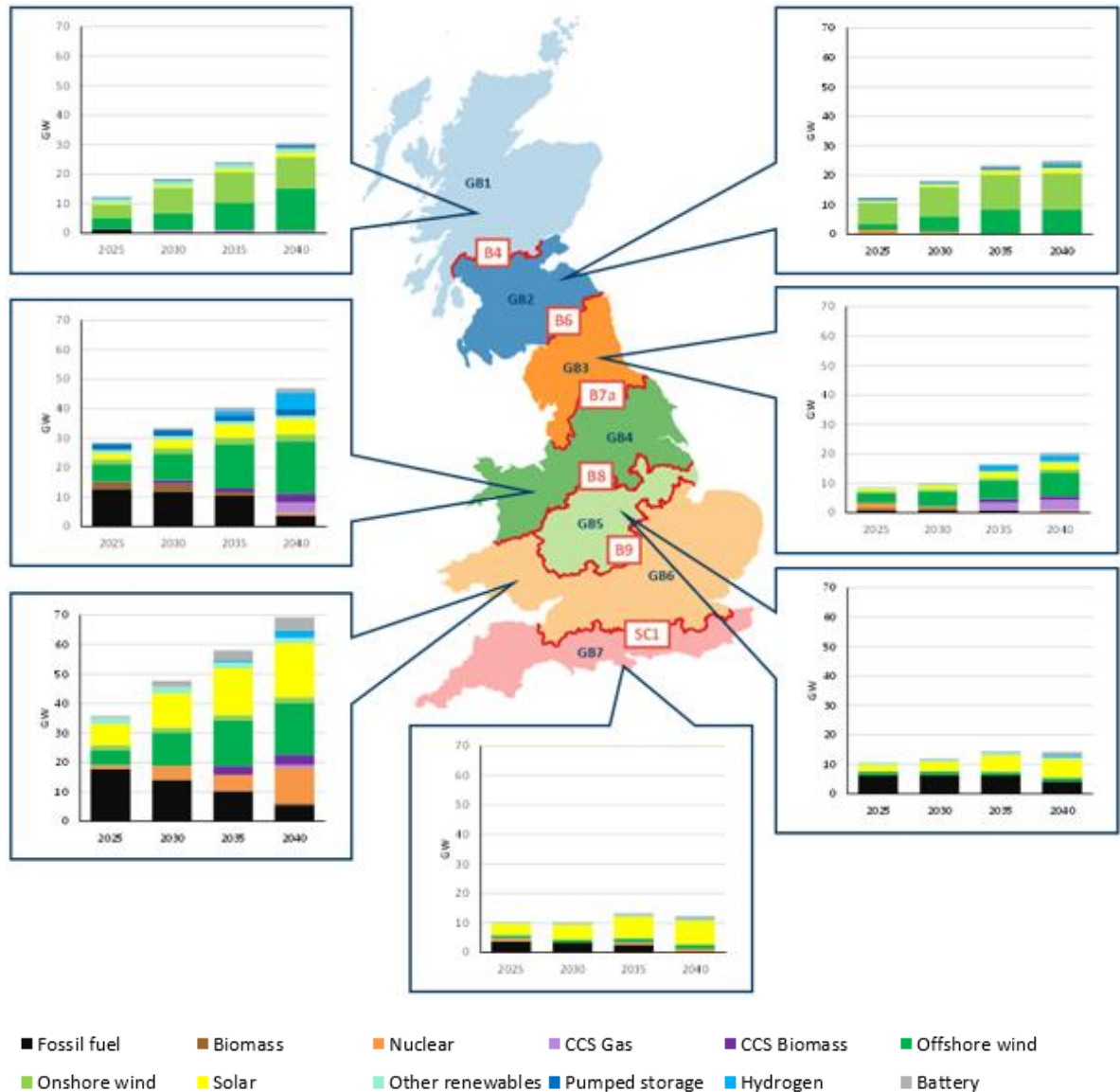
Figure A2-2: Installed capacity grouped by zone under the national market - SysTr (NOA7)
