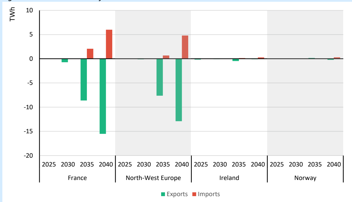
Figure 6-16: Interconnector flows in the BM
